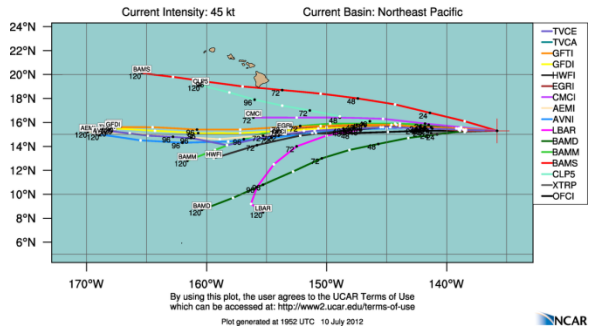
Figure 3 – Hurricane track “Spaghetti Chart” [14]
