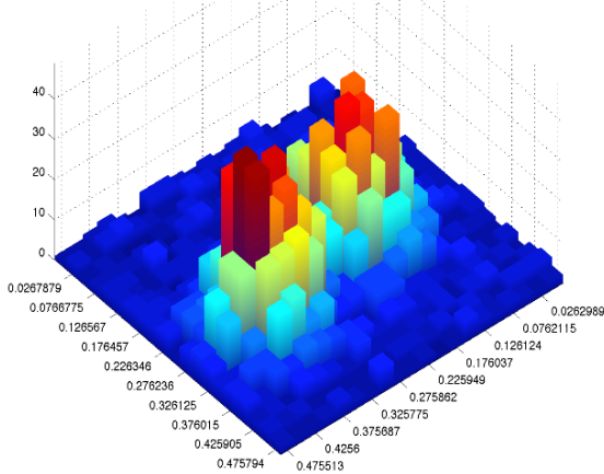
Figure 4 - 3-D Histogram via Mat Lab [15]
