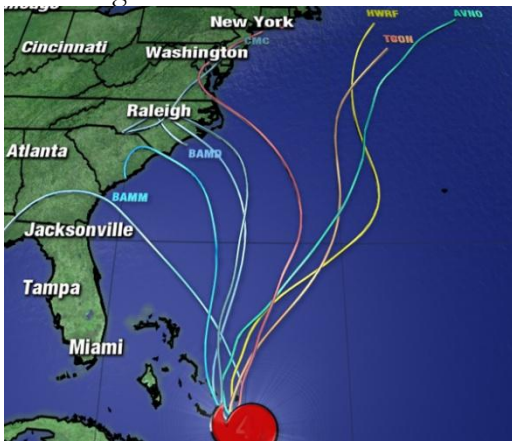
Figure 5 – Hurricane track “Spaghetti Chart” 15
