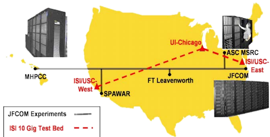
Figure 4 - USC-enabled Trans-continental Network Testbed. Maui to Virginia round trip latencies: 204 msec
